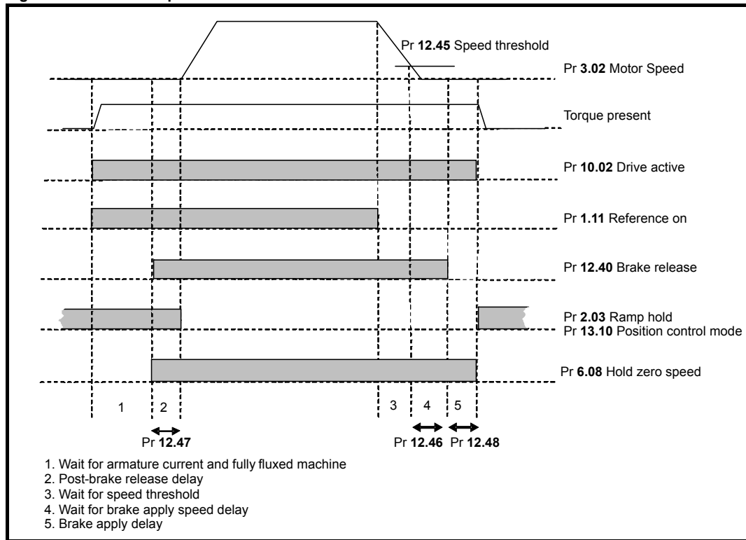
Figure 5-21 Brake sequence
