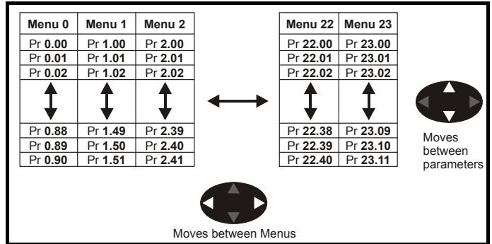
Figure 5-26 Menu structure
