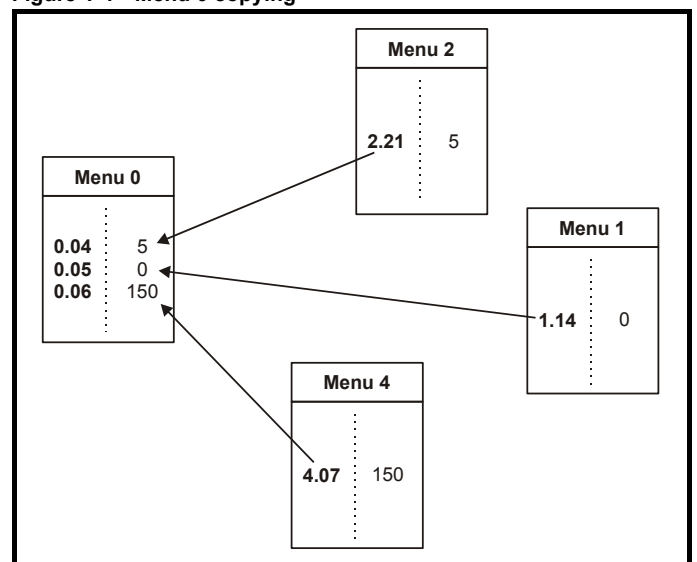
Figure 1-4 Menu 0 copying
