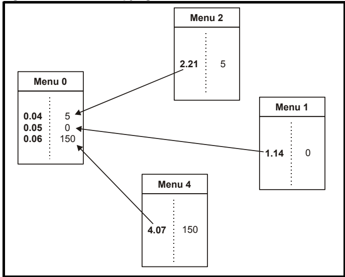
Figure 5-25 Menu 0 copying
