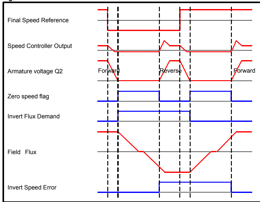
Figure 5-8 Field reversal
