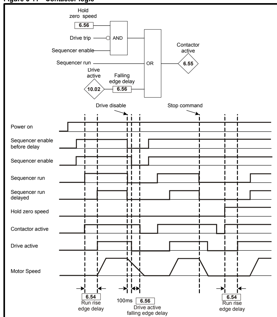
Figure 5-11 Contactor logic
